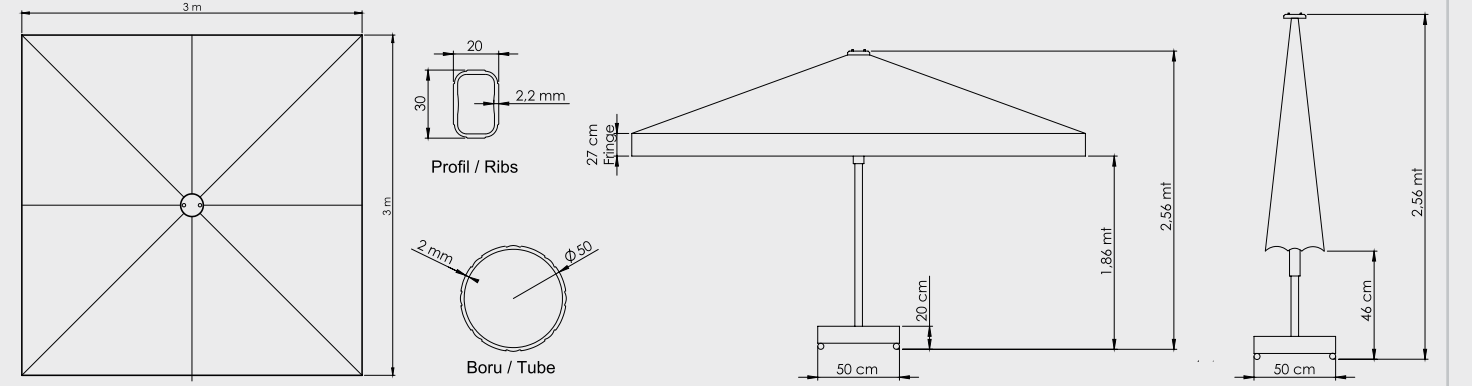
Avokado Klips Kare 300x300/8 Avocado Clips Square 300x300/8
