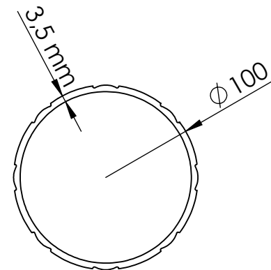
Boru / Tube
