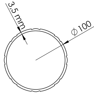
Boru / Tube
