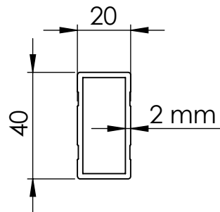
Profil / Ribs
