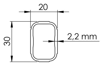
Profil / Ribs
