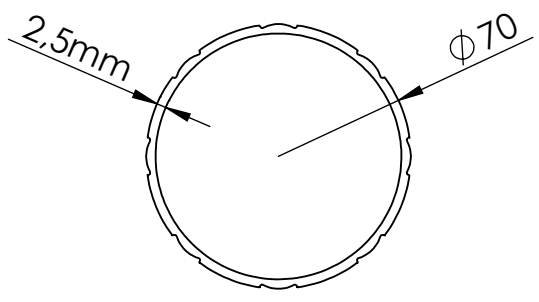
Boru / Tube
