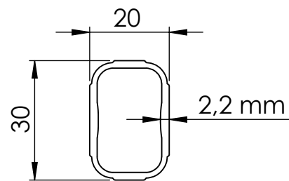
Profil / Ribs
