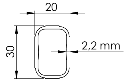
Profil / Ribs
