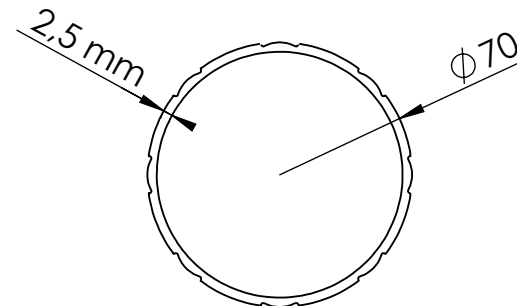
Boru / Tube
