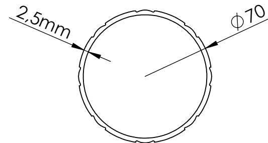
Boru / Tube
