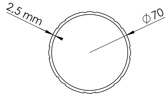
Boru / Tube
