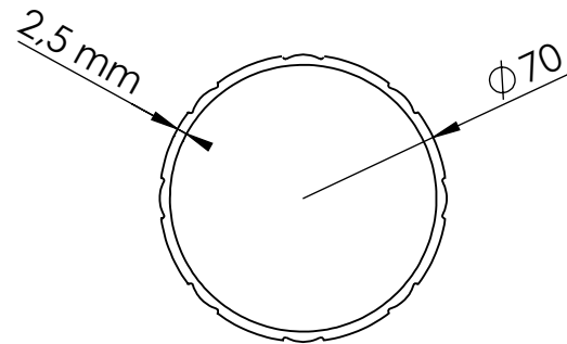
Boru / Tube
