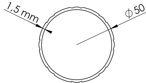
Boru / Tube
