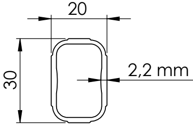
Profil / Ribs
